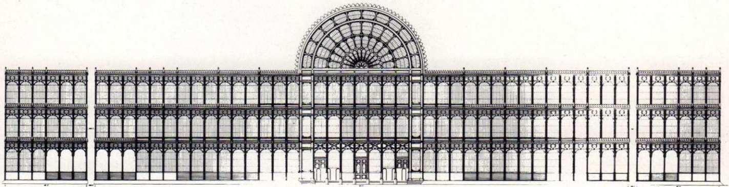
CRYSTAL PALACE. SOUTH ELEVATION
